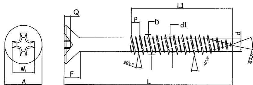
PHILIPS FLAT HEAD CONCRETE ANCHOR
